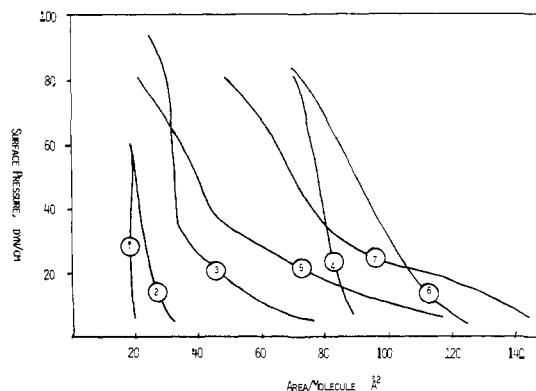
Figure 1. Surface pressure-area isotherms at 21.5 °C: curve 1, arachidic acid; curve 2, compound 3b; curve 3, sample 5a; curve 4, sample 5c; curve 5, unpurified 5; curve 6, compound 8; curve 7, purified 5b.
