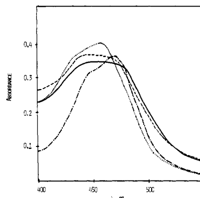
Figure 6. Spectral changes in absorption spectra occurring on irradiation of 8 in OT micelles: (· · ·) chloroform solution of 8 ; (—) monolayer assembly of 8 ; (---) micellar solution of 8-OT in water before irradiation; (- · - ·) micellar solution of 8-OT after irradiation.
